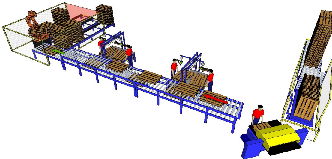
Work bench with pallet slide
